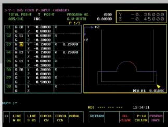
DRESS FORM INPUT SCREEN
