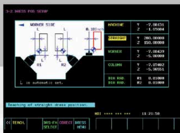
WHEEL DRESS SETUP SCREEN
