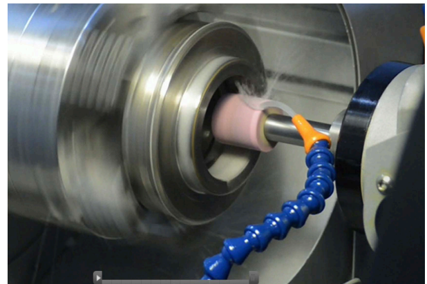
ID Wheel Attachment
