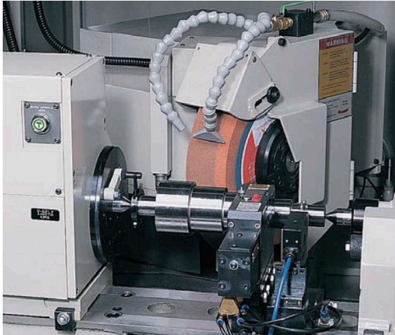
OD Grinder w/ Angle Wheel Option
